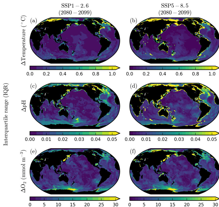
Figure A3. The interquartile range associated with CMIP6 projections of benthic impact drivers. The CMIP6 interquartile range ( Q_3 - Q_1 ) of projected anomalies in benthic (a, b) temperature ( ^{\circ}\text{C} ), (c, d) pH, and (e, f) dissolved \text{O}_2 concentration ( \text{mmol m}^{-3} ). The corresponding mean projections are given in Fig. 8.
