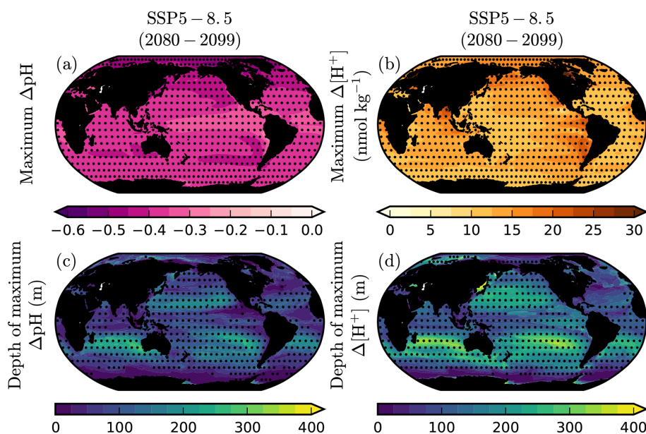
Figure 9. Magnitude and depth of maximum pH and [H^+] change under SSP5-8.5. The CMIP6 ensemble mean maximum change in (a) pH and (b) [H^+] in 2080–2099 of SSP5-8.5 relative to 1995–2014. The mean depth at which the maximum (c) pH and (d) [H^+] change is projected. Stippling designates robustness, as defined by the mean anomaly exceeding the inter-model SD.
