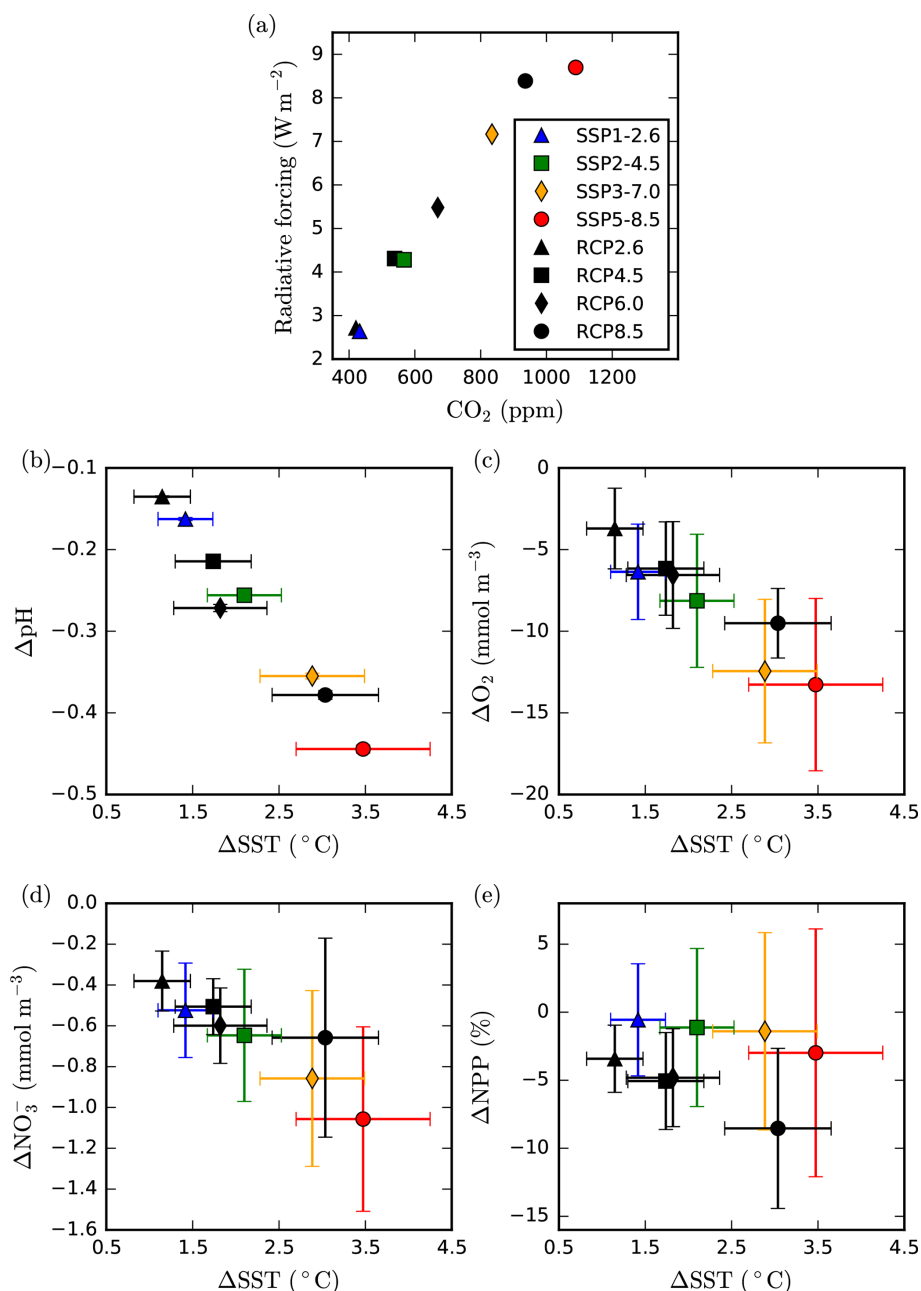
Figure 6. Comparison between CMIP6 and CMIP5 end-of-century changes in upper-ocean impact drivers. (a) Atmospheric \text{CO}_2 concentration and radiative forcing derived from the MAGICC6 model in year 2100 for the CMIP6 SSPs and CMIP5 RCPs. (b–e) Global mean anomalies of (b) surface ocean pH, (c) subsurface dissolved \text{O}_2 concentration (averaged between 100 and 600 m; \text{mmol m}^{-3} ), (d) \text{NO}_3^- concentration (averaged between 0 and 100 m; \text{mmol m}^{-3} ), and (e) integrated net primary production (%) against anomalies of sea surface temperature ( ^{\circ}\text{C} ). Anomalies are 2080–2099 mean values relative to the 1870–1899 baseline period. Error bars represent the inter-model SD.
