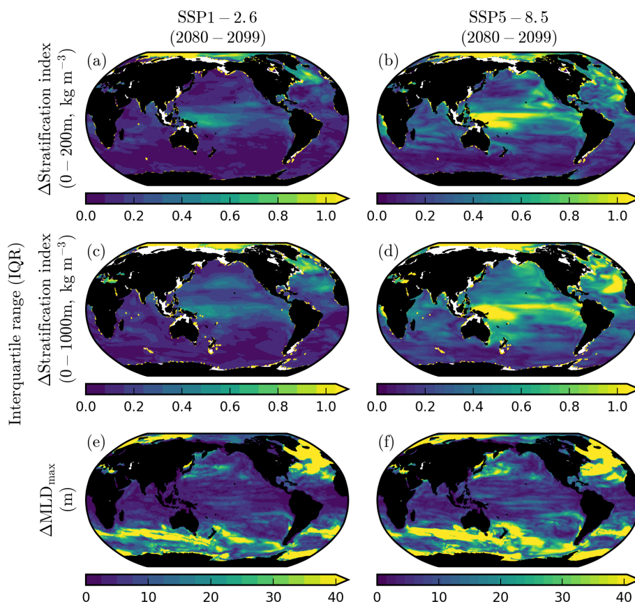
Figure A2. The interquartile range associated with CMIP6 projections of stratification and mixed-layer depth. The CMIP6 interquartile range ( Q_3 - Q_1 ) of projected anomalies in (a, b) the stratification index between 200 m and the surface ( \text{kg m}^{-3} ), (c, d) the stratification index between 1000 m and the surface ( \text{kg m}^{-3} ), and (e, f) the maximum annual mixed-layer depth (m). The corresponding mean projections are given in Fig. 4.
