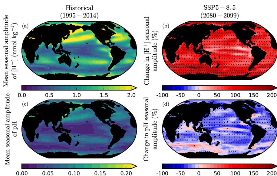
Figure 10. Change in the seasonal amplitude of surface ocean [H^+] and pH. The CMIP6 historical climatologies and SSP5-8.5 anomalies in peak-to-peak seasonal amplitude of surface ocean (a, b) [H^+] and (c, d) pH. Anomalies are calculated from the mean seasonal amplitude in 2080–2099 relative to that in 1995–2014. Stippling designates robustness, as defined by at least 80 % model sign agreement.
